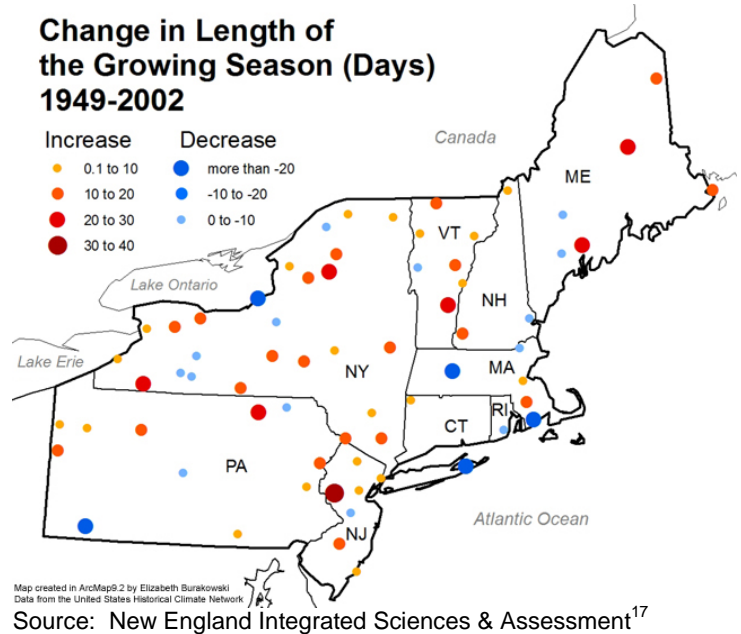
Figure 7 – Growing Season Has Increased
